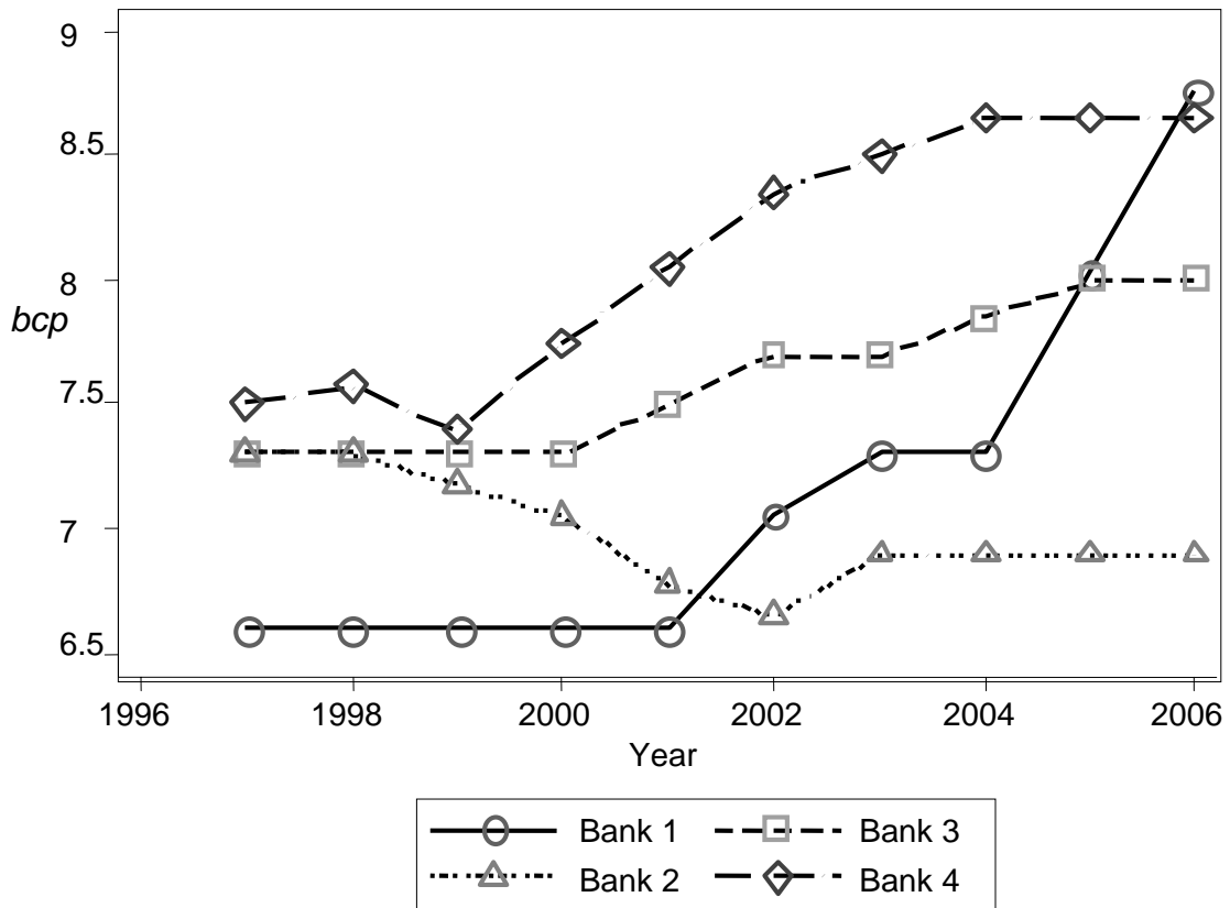
Figure 1: Trends in bcp by Bank
